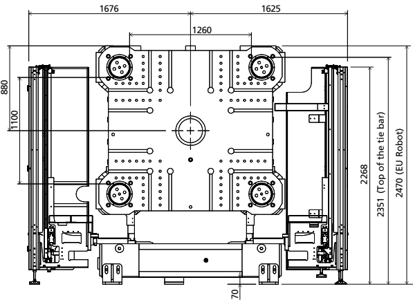
Mechanical interface
